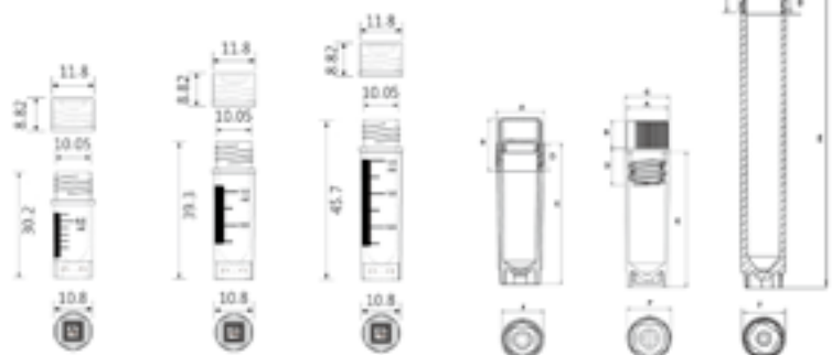
Dimensions = mm
