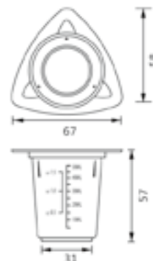
Dimensions = mm
