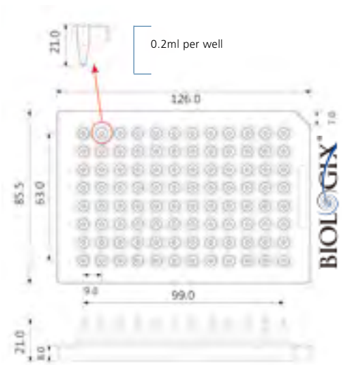
Dimensions = mm
