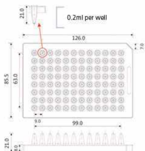
Dimensions = mm
